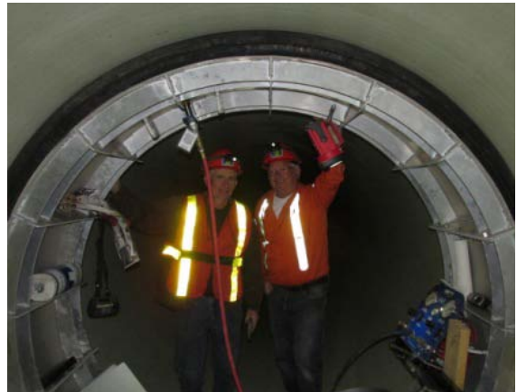
Photo 20 – Pressure testing the penstock
