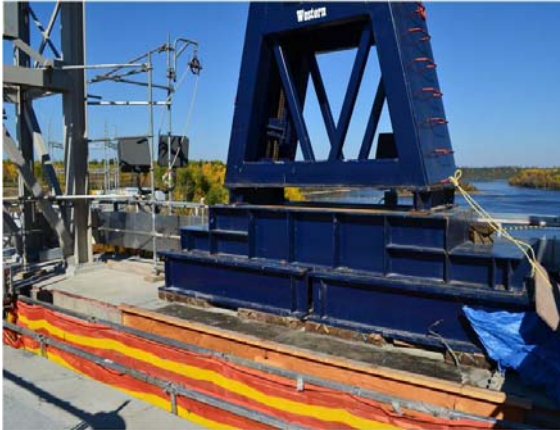
Photo 17 – Repairing the intake gate concrete
