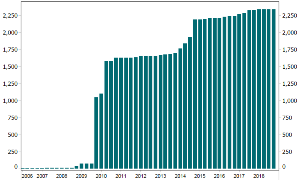
Figure 20: Hydroelectric Capacity Added into Service by Quarter/Year
