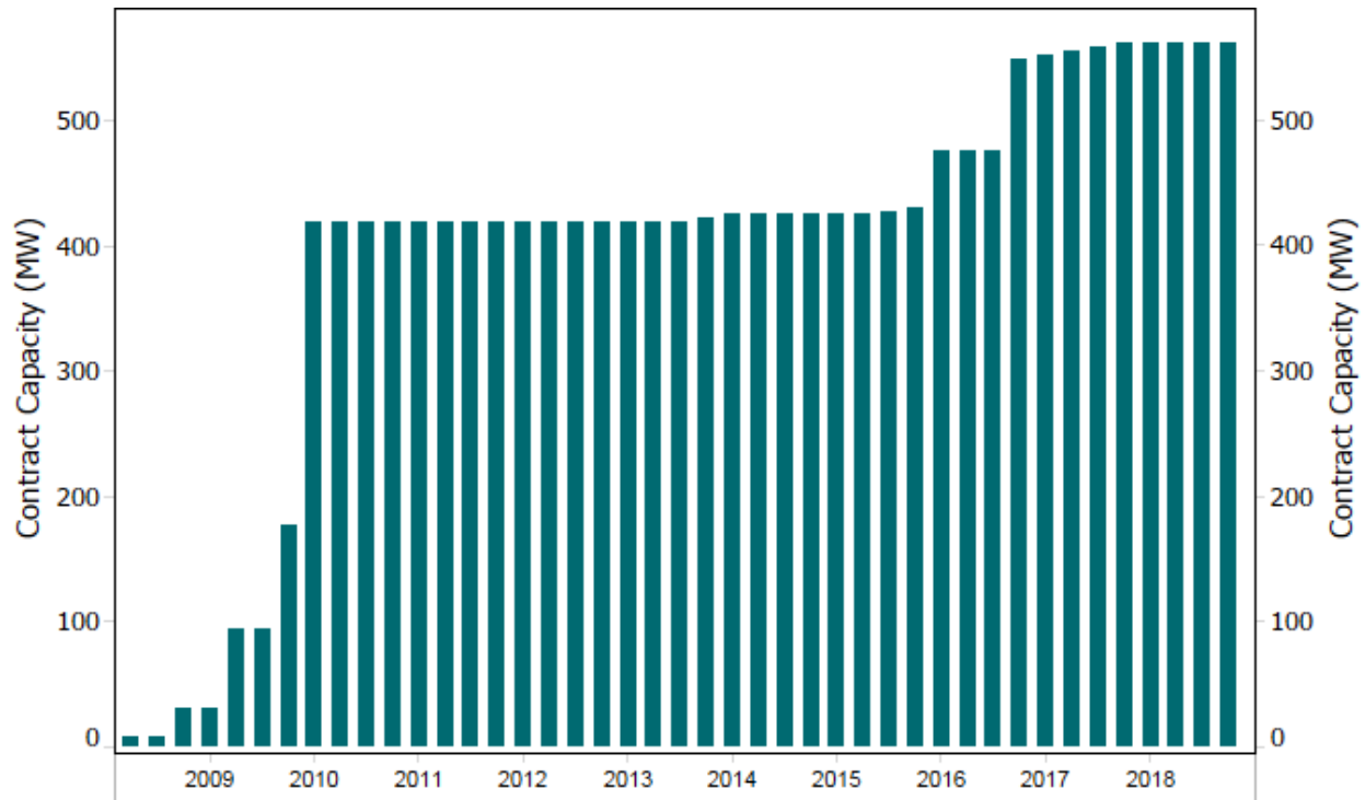
Figure 15: Cogeneration – Natural, By-Product Gas Capacity Added into Service by Quarter/Year
