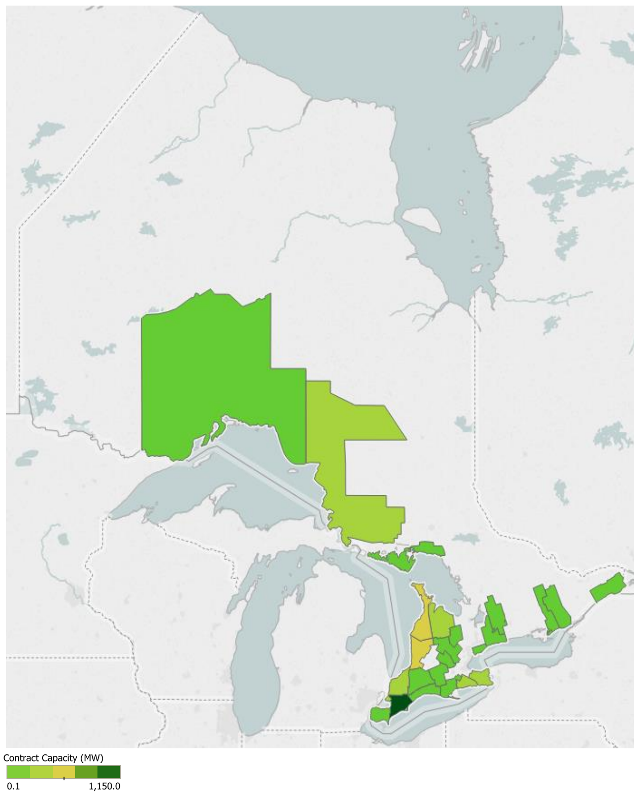
Figure 28: Map of Wind Capacity In-Service
