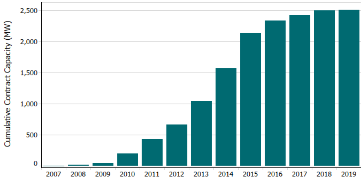
Figure 23: Solar Capacity Added into Service by Year
