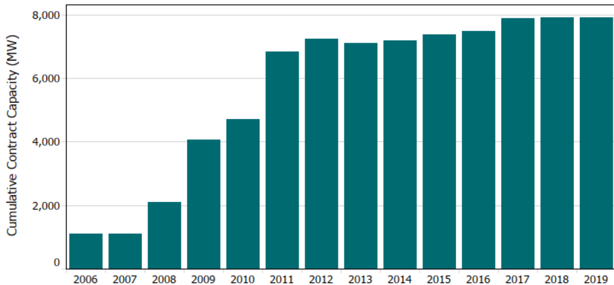
Figure 14: SC/CC - Natural Gas Capacity Added into Service by Year
