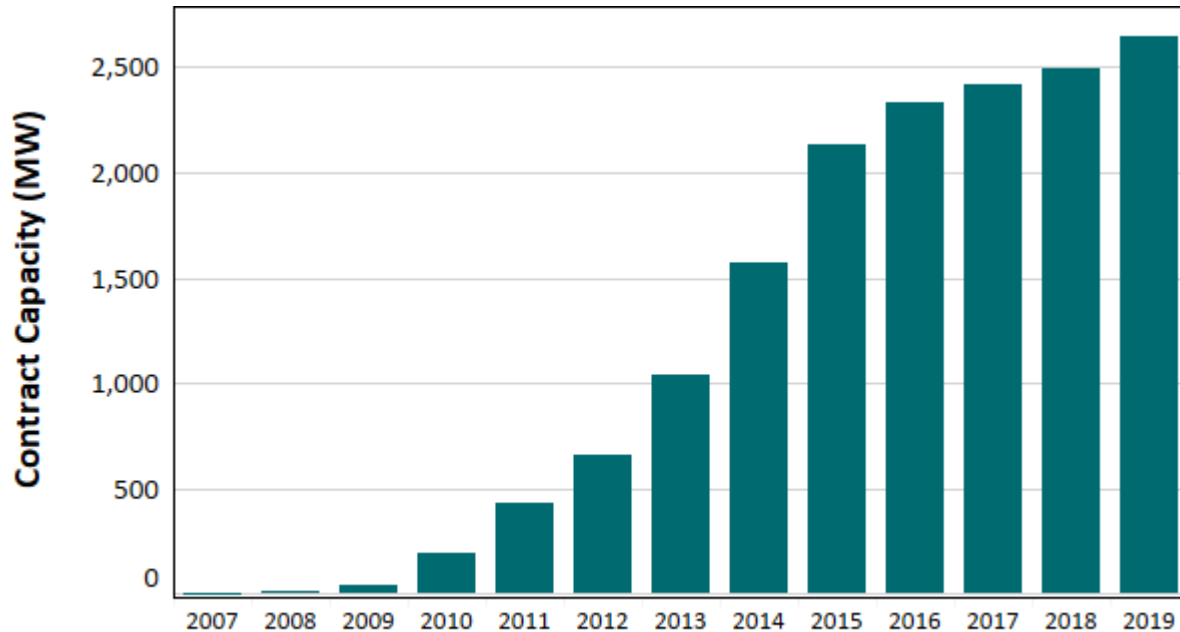
Figure 22: Solar Capacity Added in Service by Year
