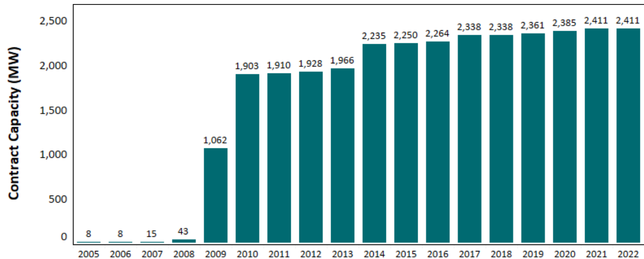
Figure 22: Solar Capacity Added in Service by Year
