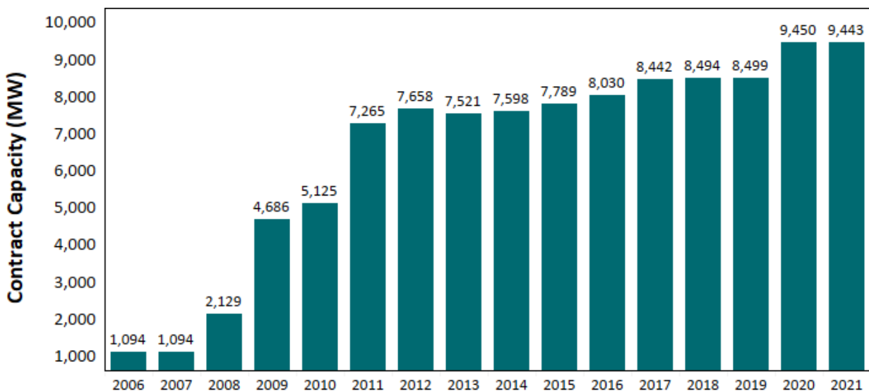
Figure 14: Gas Capacity Added in Service by Year
