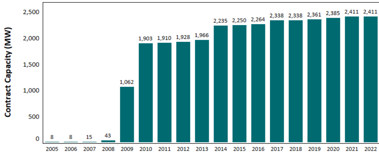
Figure 19: Hydroelectric Capacity Added in Service by Year
