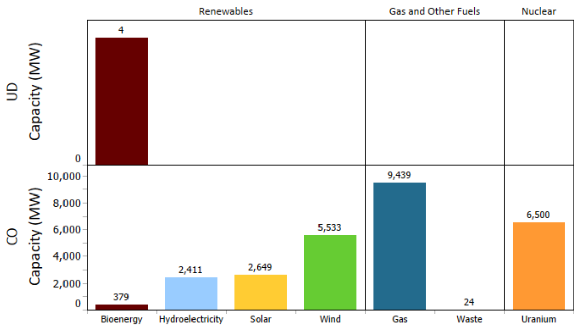
Figure 2: Total Contracted Capacity by Contract Status
