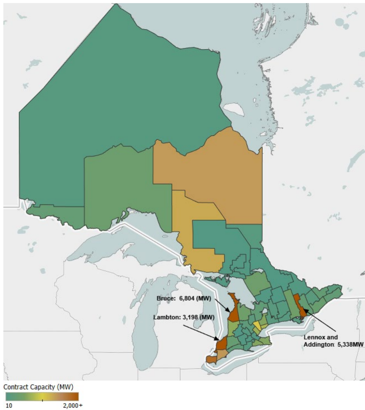
Figure 3: Map of Total Contracted Capacity in Ontario
