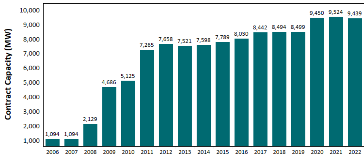
Figure 14: Gas Capacity Added in Service by Year
