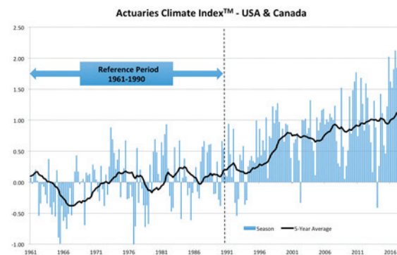
Figure 1.5. Changes in the frequency of climate extreme events that have occurred across North America since 1961 as measured by the Actuarial Climate Index. The index measures changes in extremes of high and low temperatures, high winds, heavy precipitation, and drought, as well as changes in sea level, expressed in units of standard deviations from the mean for the 30-year reference period of 1961-1990.
