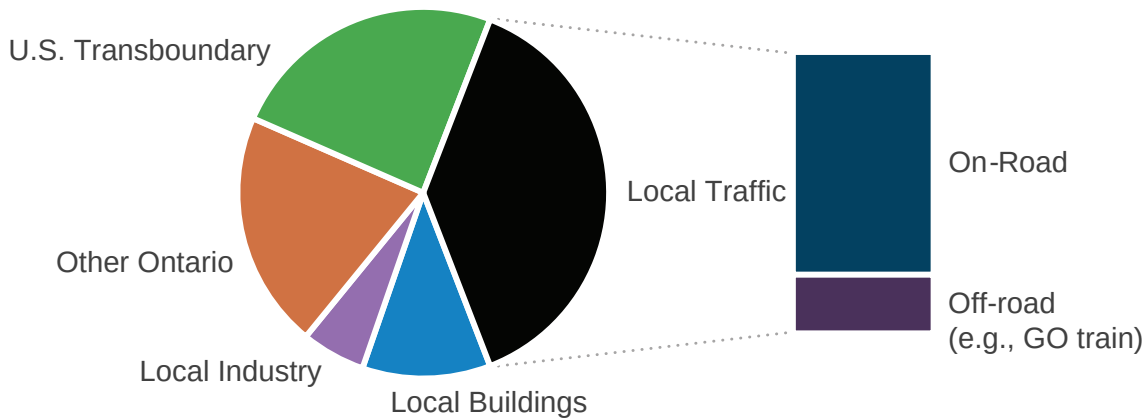
Figure 3.22. Causes of of air pollution related hospitalizations in Toronto.
