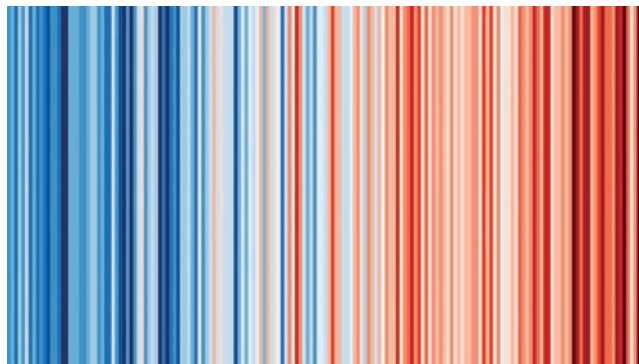
Annual temperatures in Toronto from 1841-2017. The colour scale goes from 7.6°C (dark blue) to 10.8°C (dark red).
