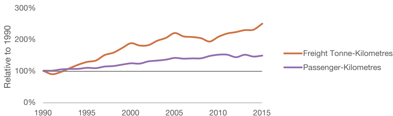
Figure 1.23. Ontario's on-road vehicle activity.
