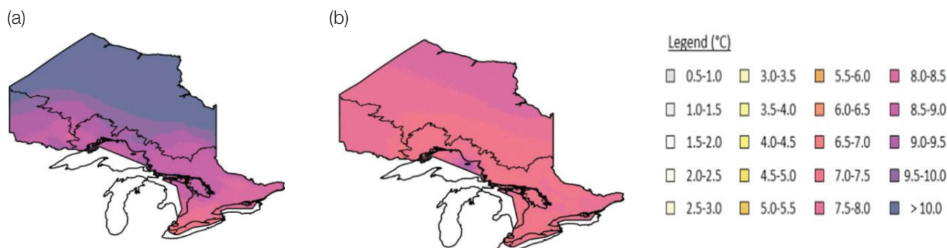
Figure 1.7. Projected change in Ontario's (a) winter temperatures and (b) summer temperatures for the years 2071-2100 relative to 1971-2000 baseline values. Note: This projection is based on representative concentration pathway 8.5 (warming expected under very high emission scenario due to failure to curb emissions by 2100).
