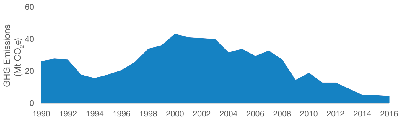
Figure 1.41. Ontario's historical greenhouse gas (GHG) emissions from electricity (in megatonnes of carbon dioxide equivalent, Mt CO 2 e).
