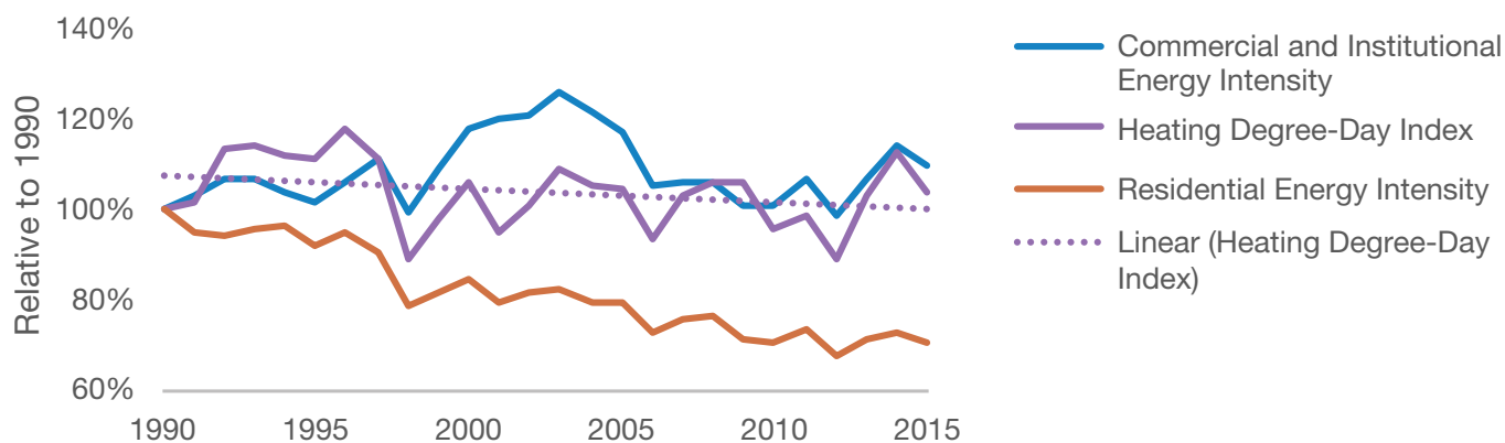
Figure 1.33. Residential buildings are getting more efficient but commercial and institutional building are not.
