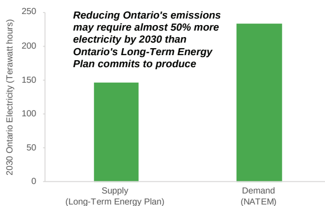
Figure 3.1. The 2030 electricity supply projected by the 2017 Long-Term Energy Plan vs. the 2030 electricity demand projected under the NATEM.
