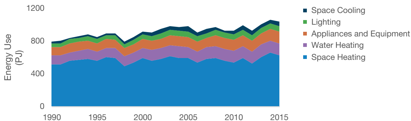
Figure 1.35. Ontario's historical building energy use by end use (in petajoules).
