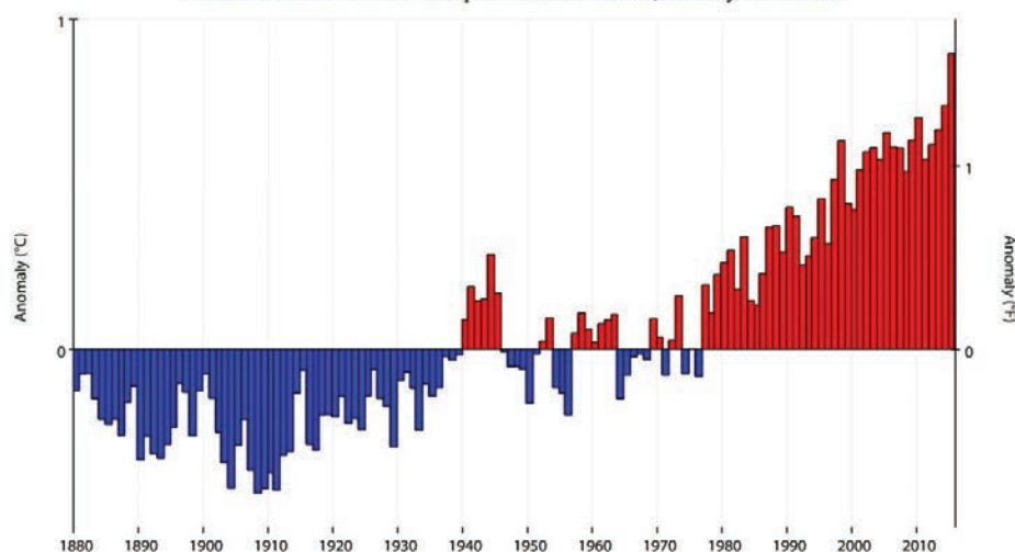
Global Land and Ocean Temperature Anomalies, January-December
