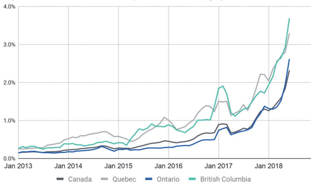
Figure B.9. Electric vehicles as a percentage of all vehicles sold in Canada and three provinces (including Ontario).
