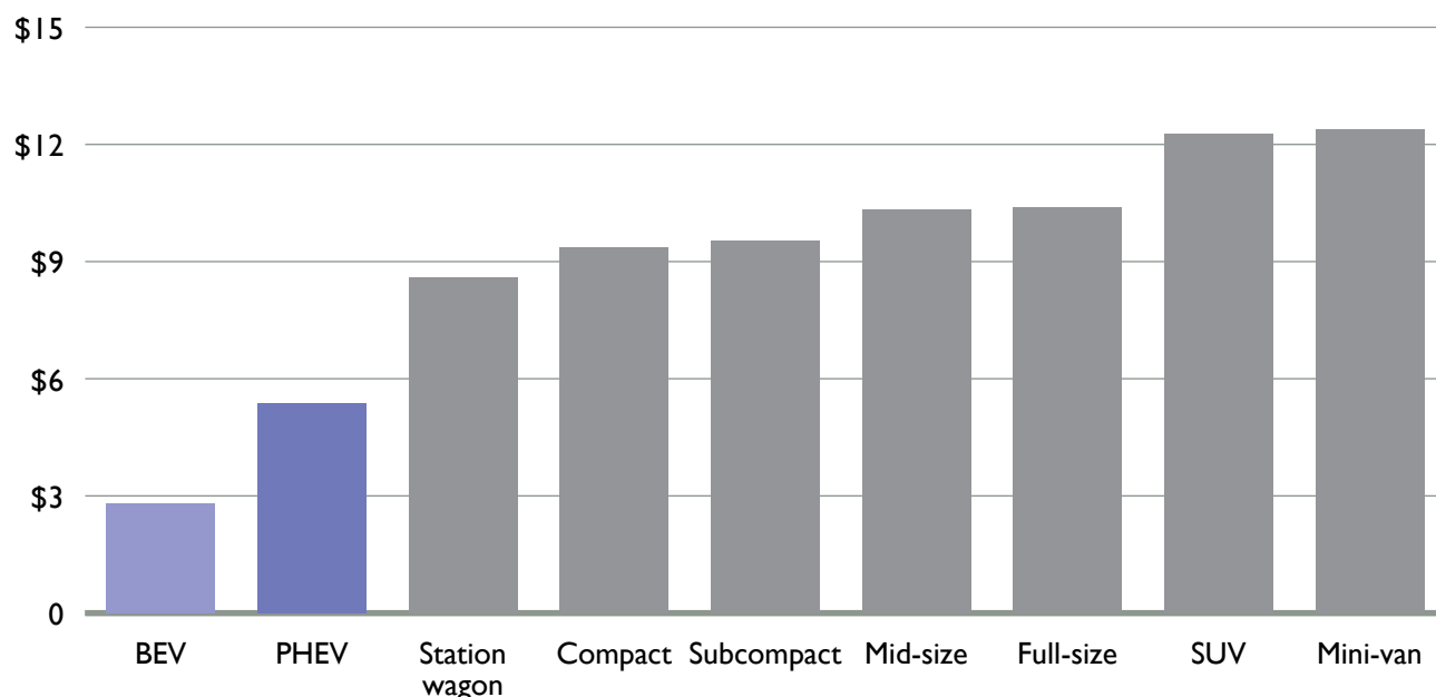
Figure 3.4: Average cost to drive 100 kilometers in Ontario (BEV – Battery Electric Vehicle; PHEV – Plug-in Hybrid Electric Vehicle)
