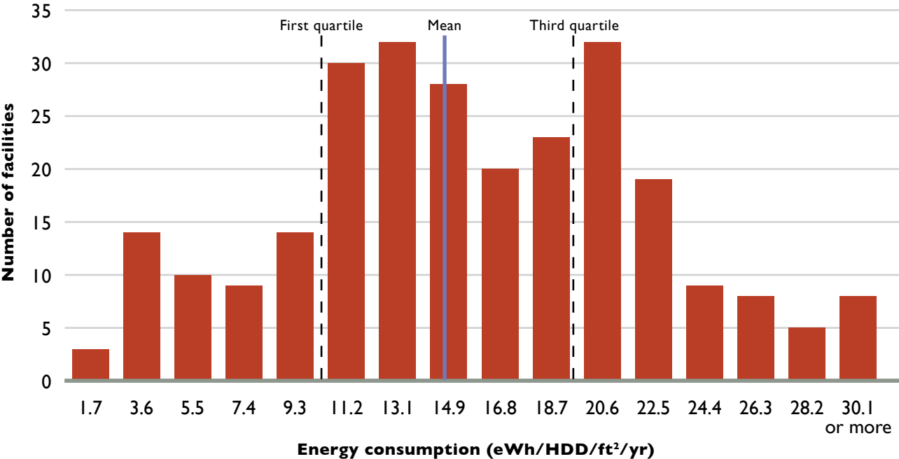
Figure 4.4: Energy consumption curve for Ontario’s hospitals – 2011
