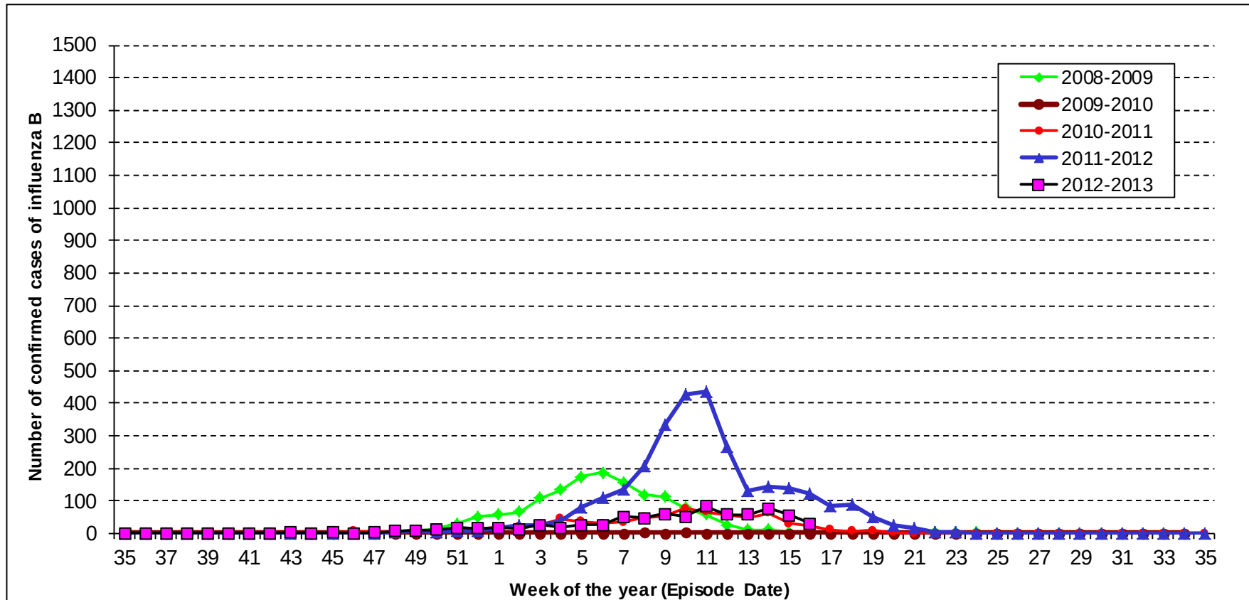
Figure 2. Number of reported confirmed cases of influenza B by episode date: Ontario, September 1, 2008 to April 20, 2013
