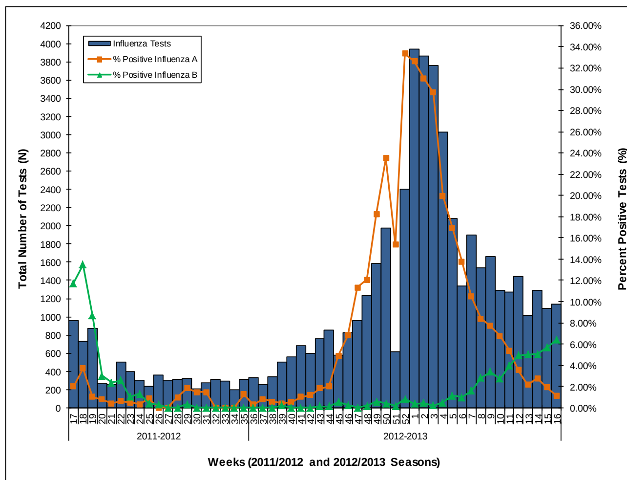
Figure I. Total number of influenza tests performed and percent of positive tests by report week: Ontario, April 22, 2012 to April 20, 2013
