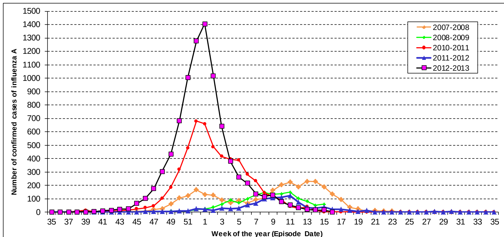
Figure 1. Number of reported confirmed cases of influenza A by episode date: Ontario, September 1, 2007 to April 20, 2013
