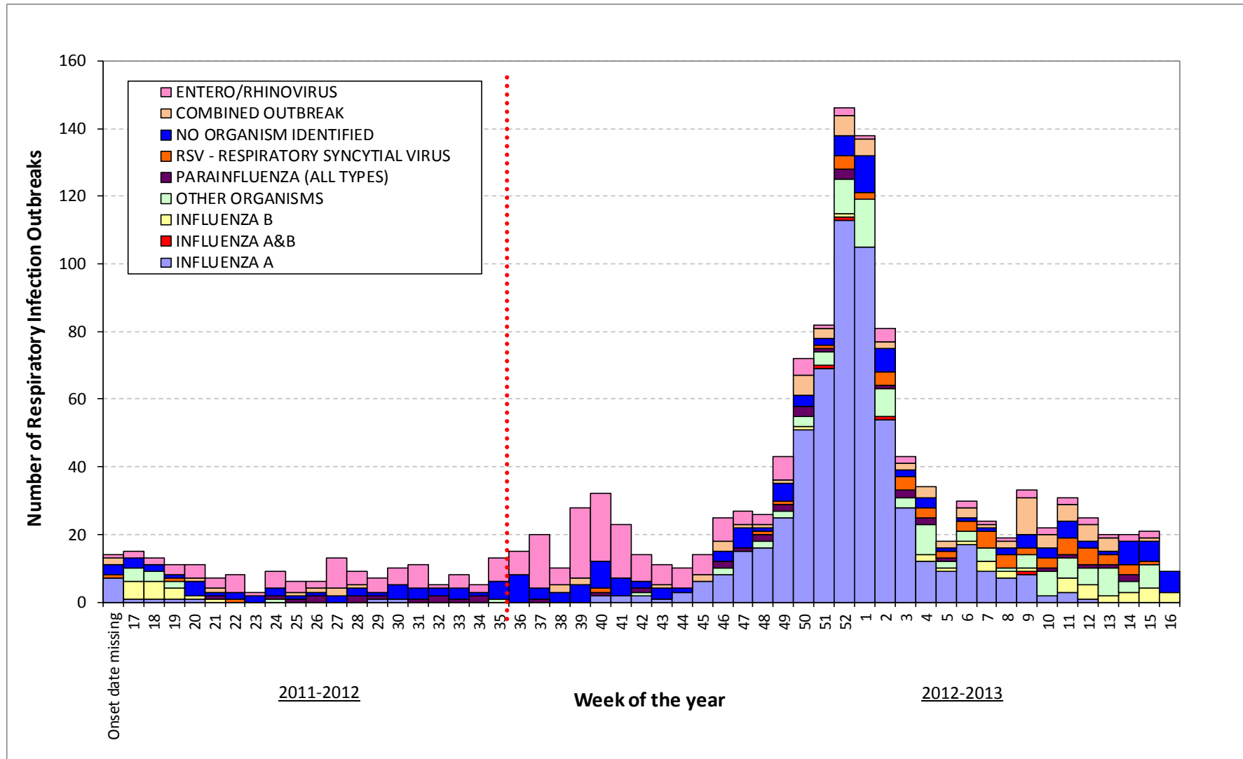
Figure 5. Institutional respiratory infection outbreaks by week of illness onset in the first case: Ontario, April 22, 2012 to April 20, 2013
