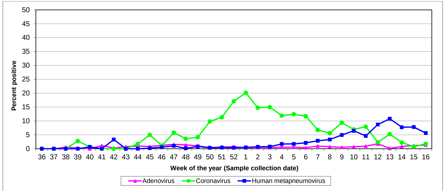
Figure 4. Percentage of respiratory viral pathogens (coronavirus, metapneumovirus, adenovirus) detected among specimens tested by all methods at PHOL: Ontario, September 2, 2012 to April 20, 2013
