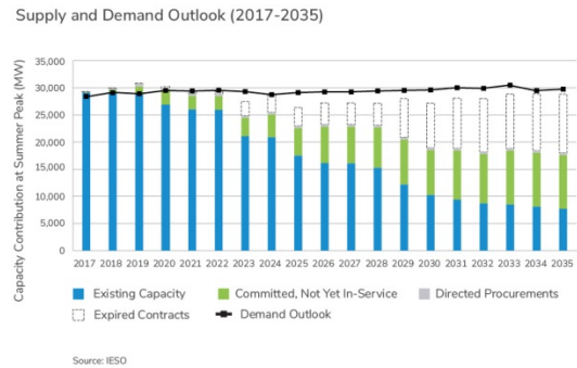
• Figure 8, Integrated Electricity Demand and Supply Outlook
