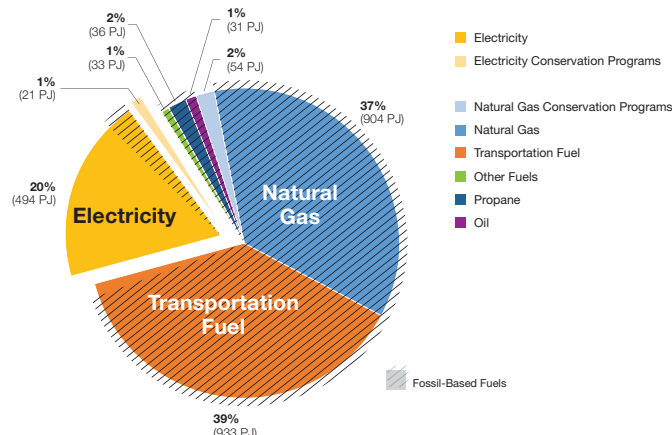
Ontario's energy use, by fuel type in 2015, including demand reduced by utility-run conservation programs.
