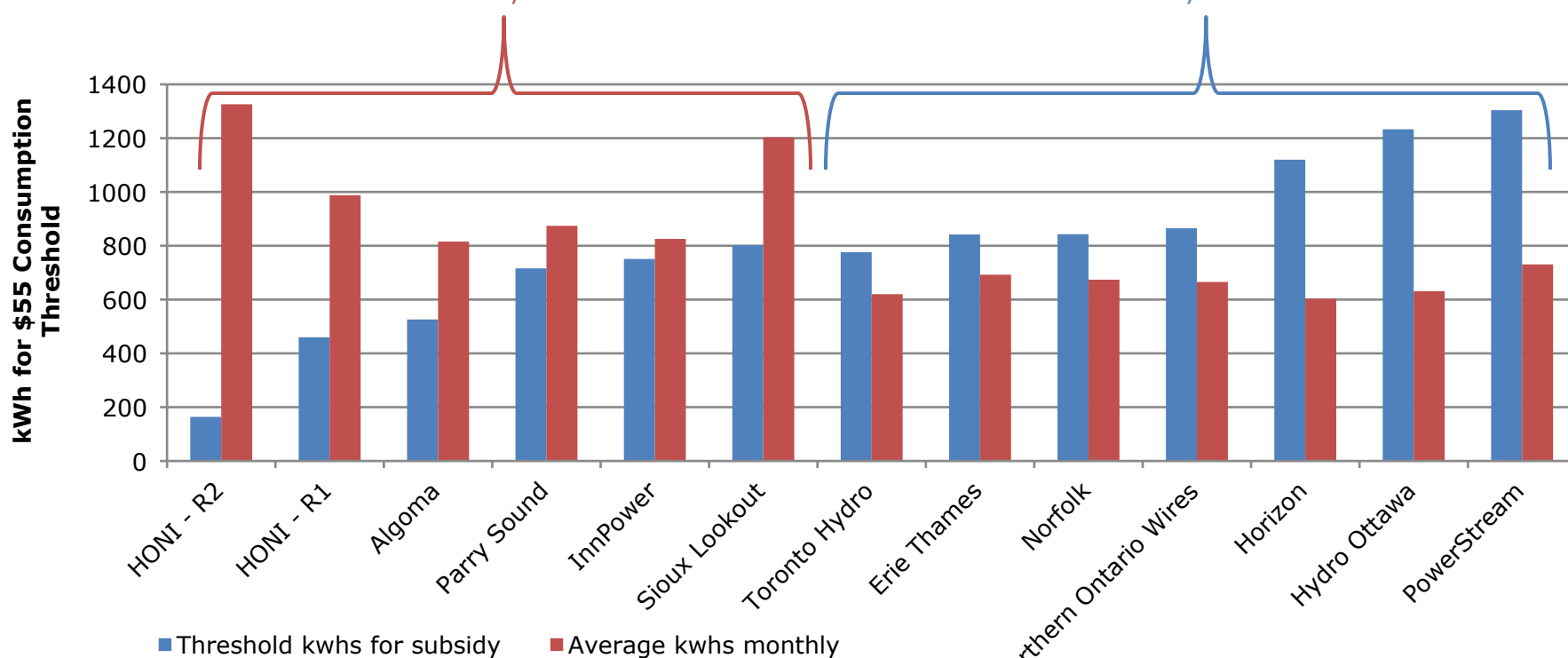
Consumption Threshold for $55 Delivery Line Subsidy vs. Average monthly kwhs – Example LDCs
