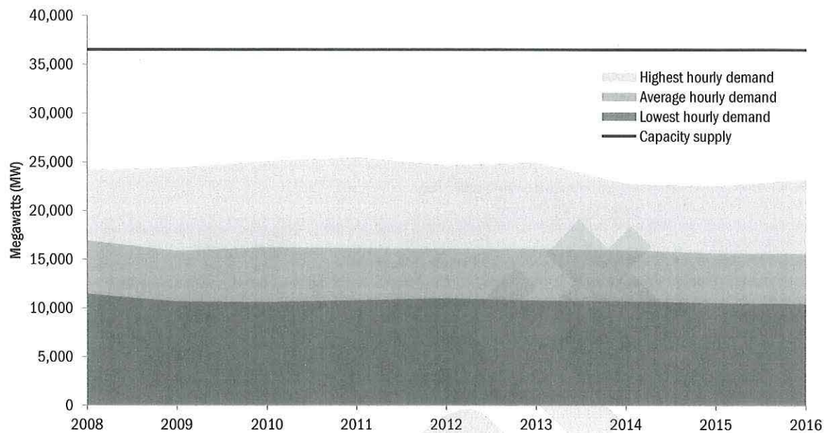
Figure 1: Ontario's Hourly Electricity Demand, 2008–2016
