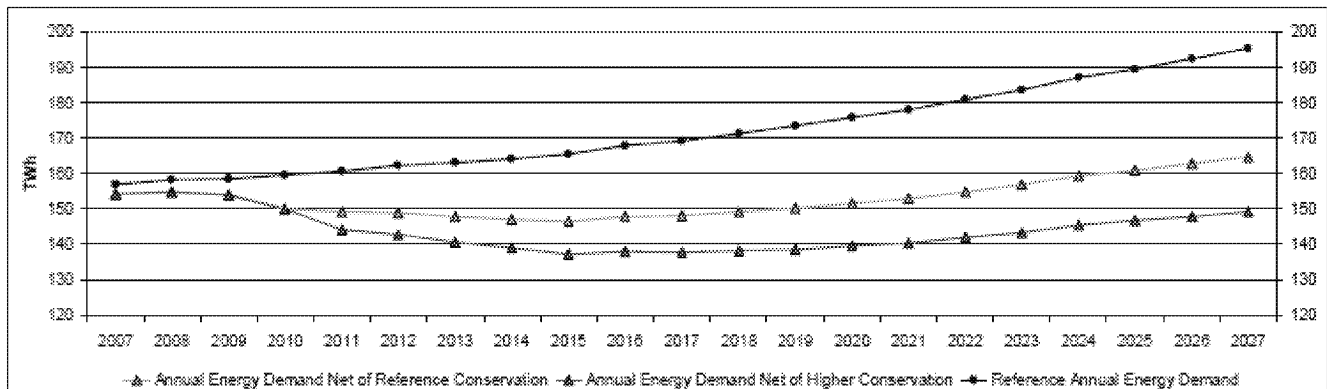
Figure 7: Annual Energy Demand under Reference and Higher Conservation Scenarios
