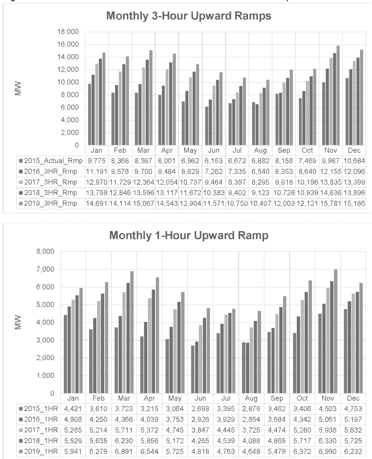
Figure 2: Forecasted Maximum Three Hour and One Hour Net Load Ramps
