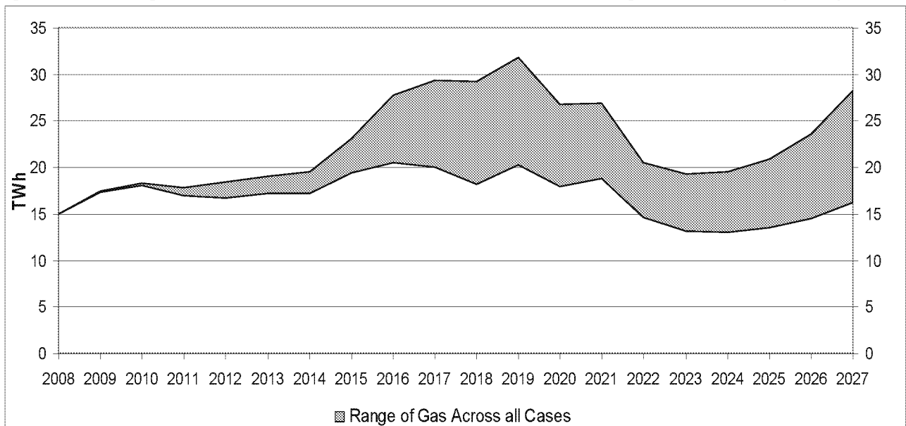
Figure 18: Range of Natural Gas-Fired Production across eight Scenarios (TWh)
