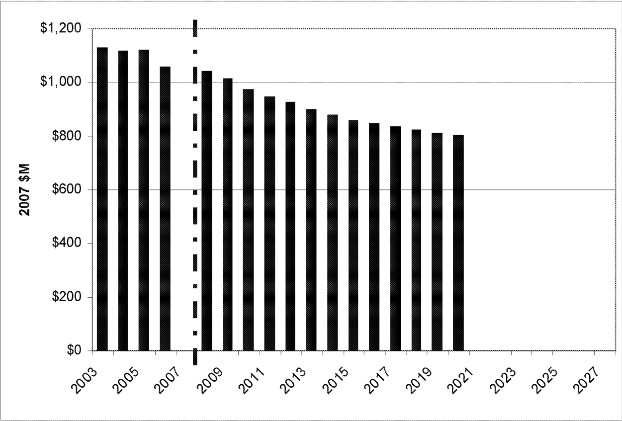
Figure 19: Cost of Debt Retirement Charge (2007 $Millions)
