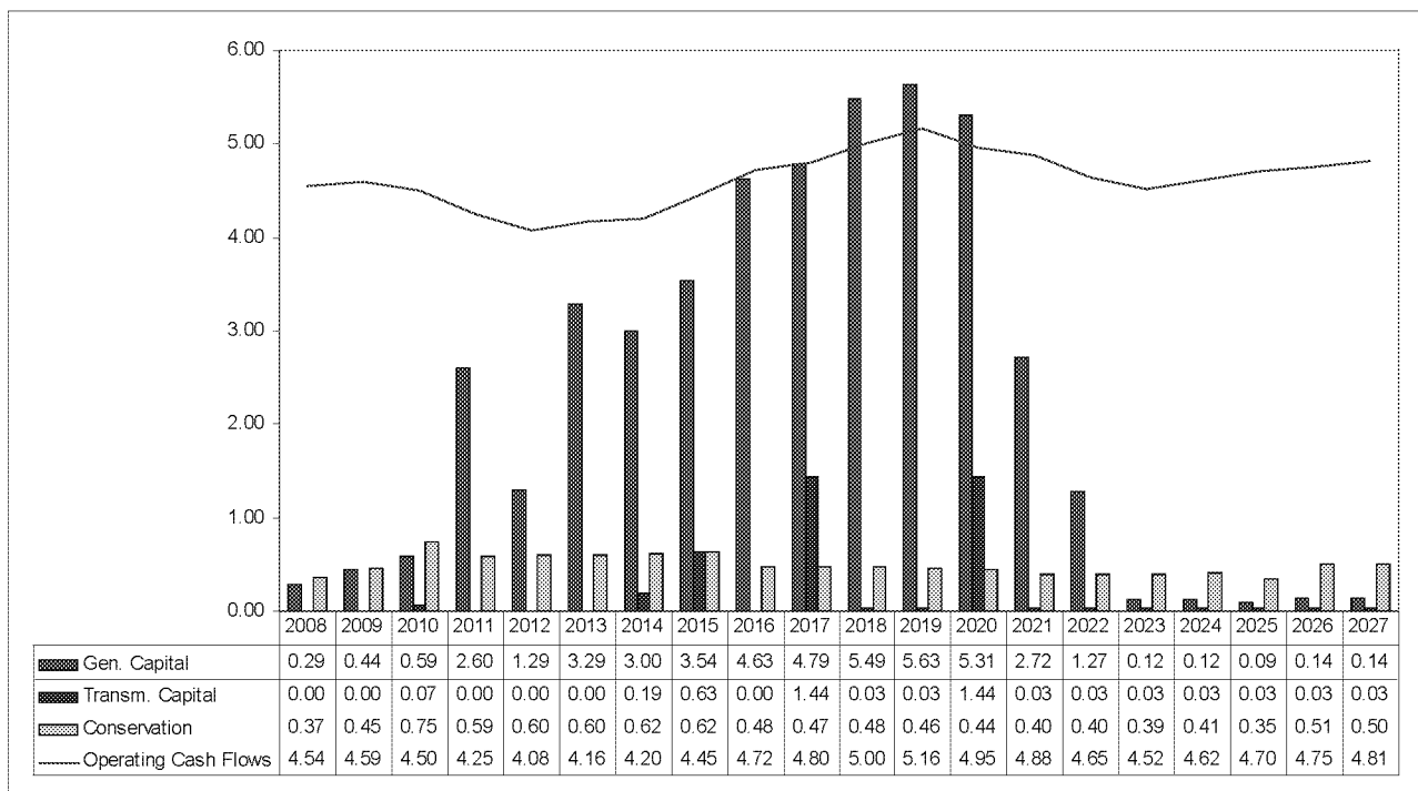
Figure 7: Case 1A Forecast Period Annual Cash Flows (2007 $Billions)
