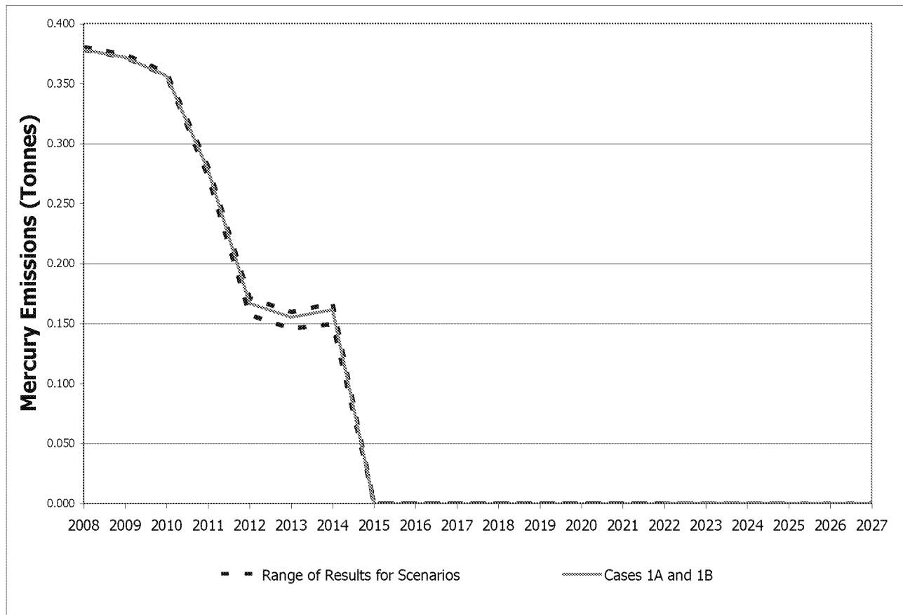
Figure 5: Summary of Mercury Emissions to Air
