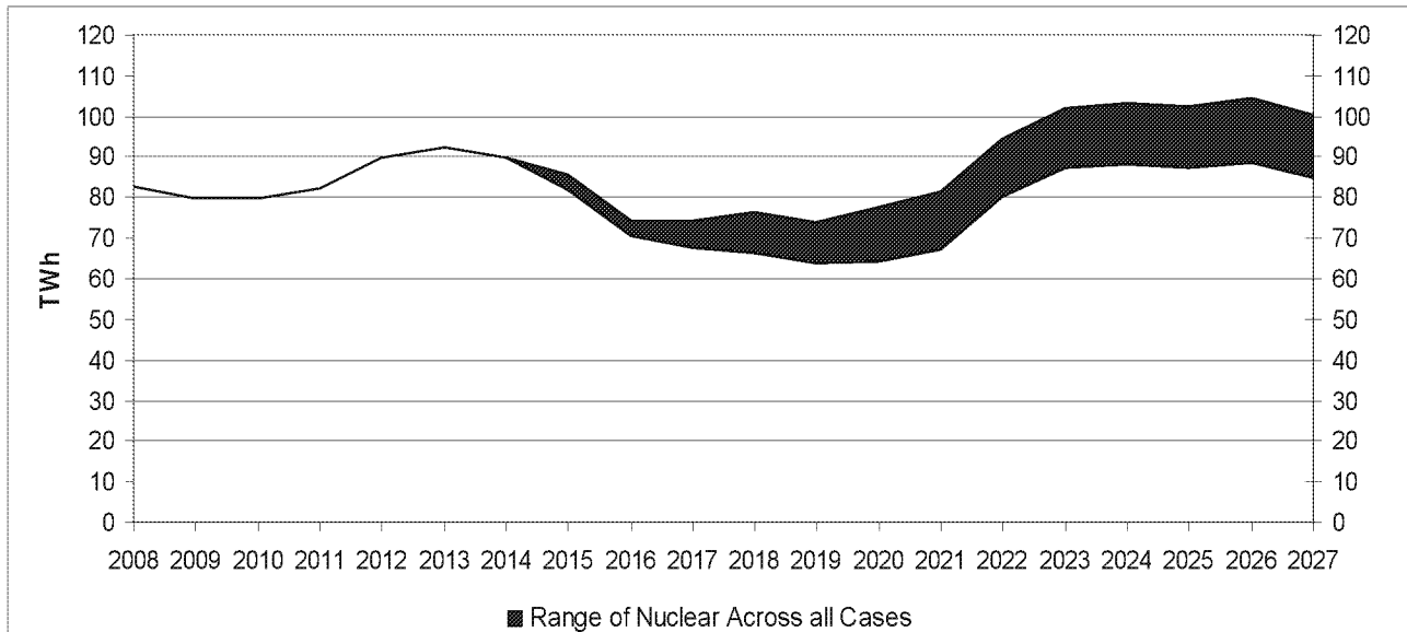
Figure 17: Range of Nuclear Production across eight Scenarios (TWh)
