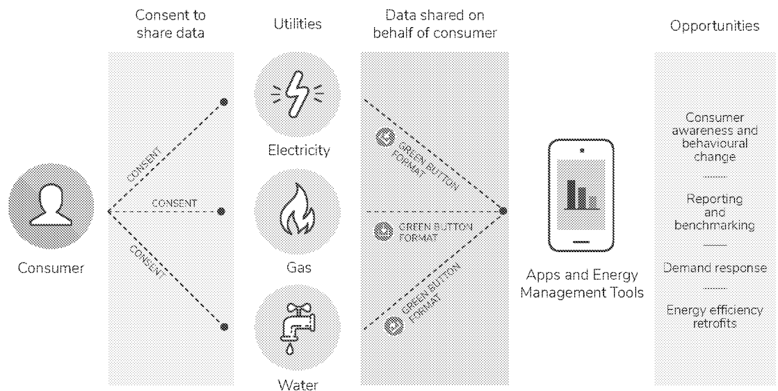
FIGURE 17. Green Button Connect My Data
