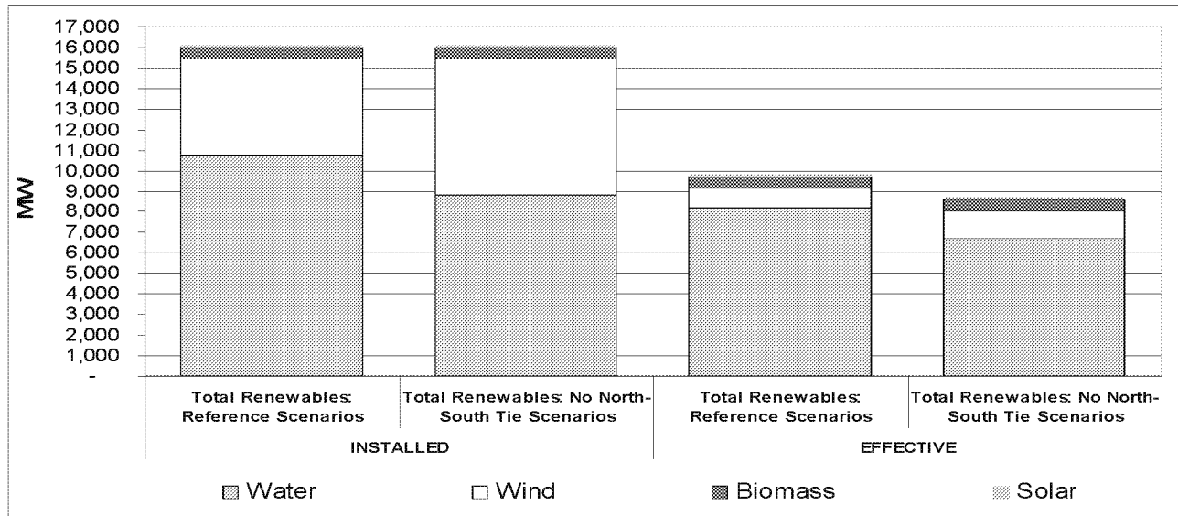
Figure 11: Comparison of Total Renewables under Reference and no-North-South Tie Scenarios (MW)
