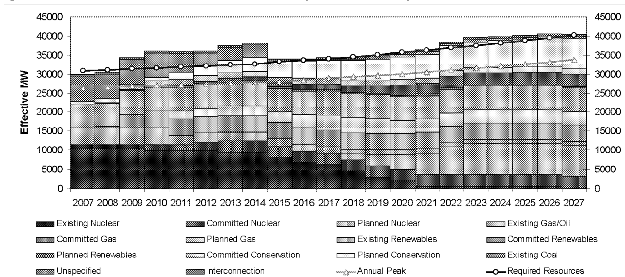
Figure 9: Case 3B Cumulative Resources (Effective MW)
