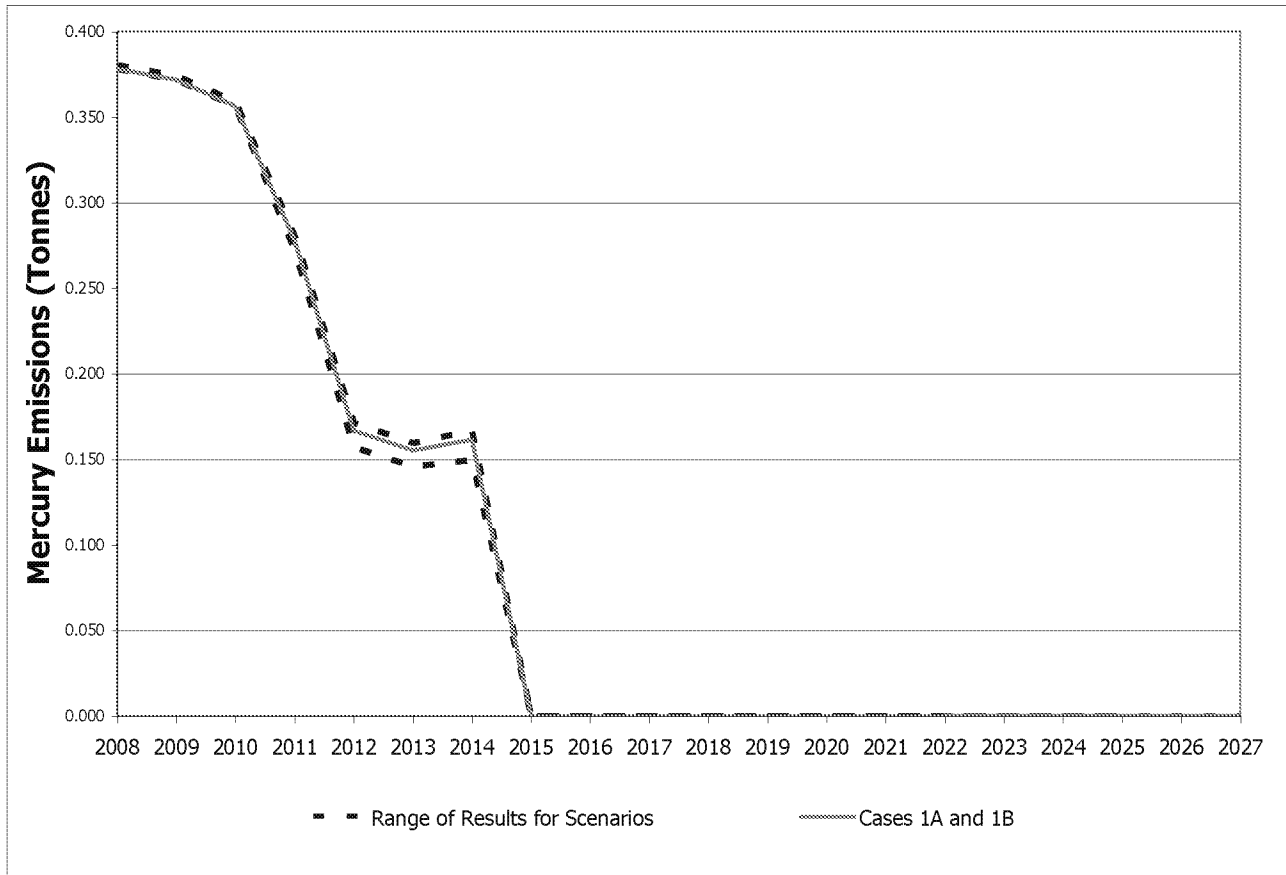
Figure 5: Summary of Mercury Emissions to Air
