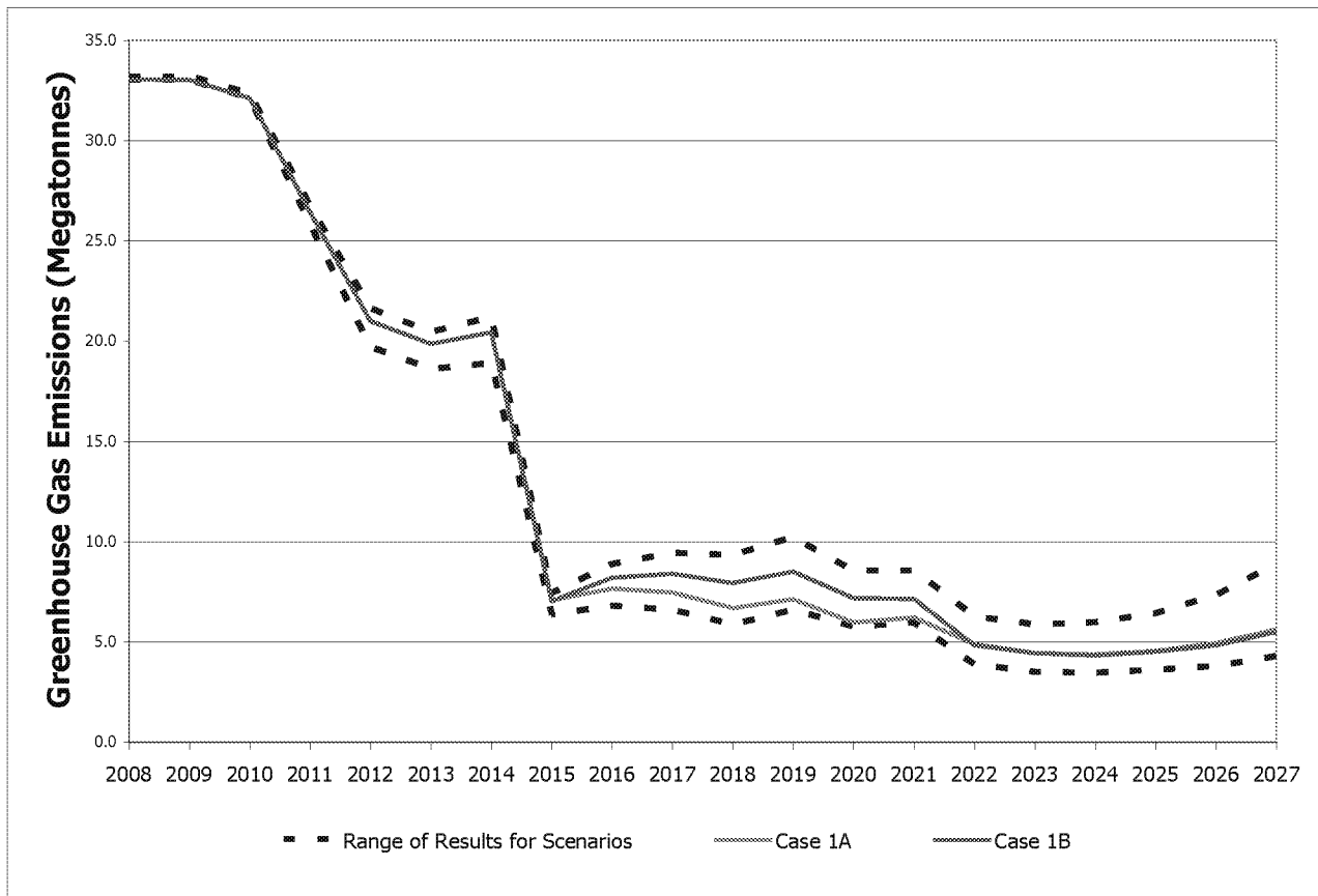
Figure 1: Summary of Greenhouse Gas Emissions
