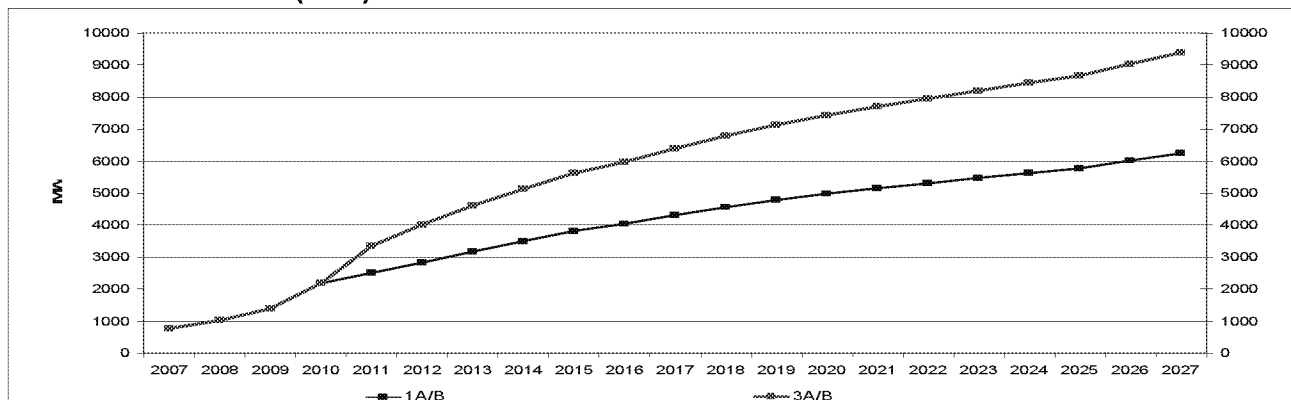
Figure 4: Comparison of Conservation under Reference and Higher Conservation Scenarios (MW)
