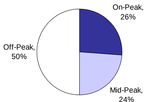
Figure 6: Breakdown of Average RPP Consumption by TOU Periods
