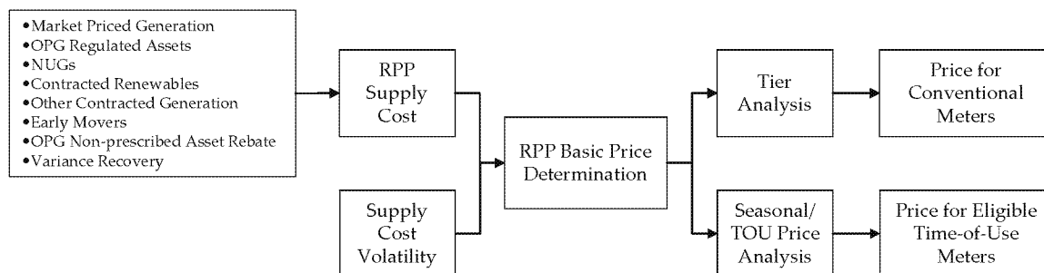
Figure 1: Process Flow for Determining the RPP Price
