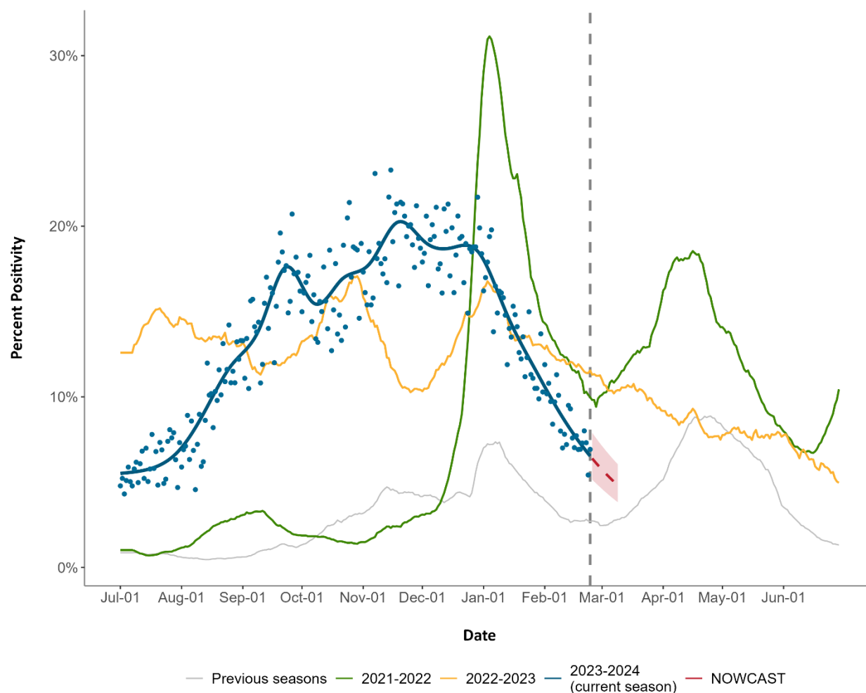
Figure 1a: Historic and projected SARS-CoV-2 activity (percent positivity) in Ontario
