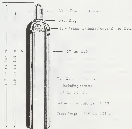
Figure 3-1 CHLORINE CYLINDERS
