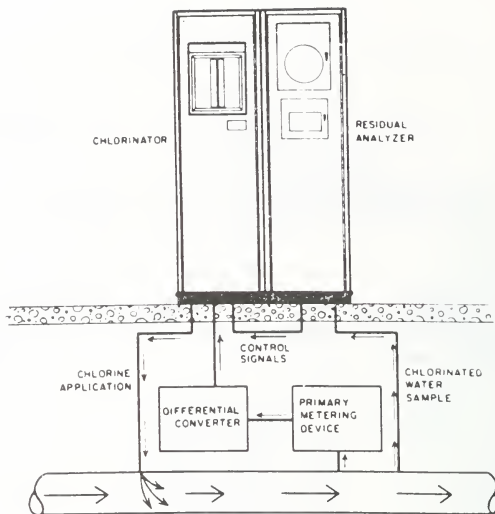
Figure 5-4 COMPOUND LOOP CONTROL
