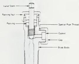
Figure 3-6 TON CONTAINER VALVE
