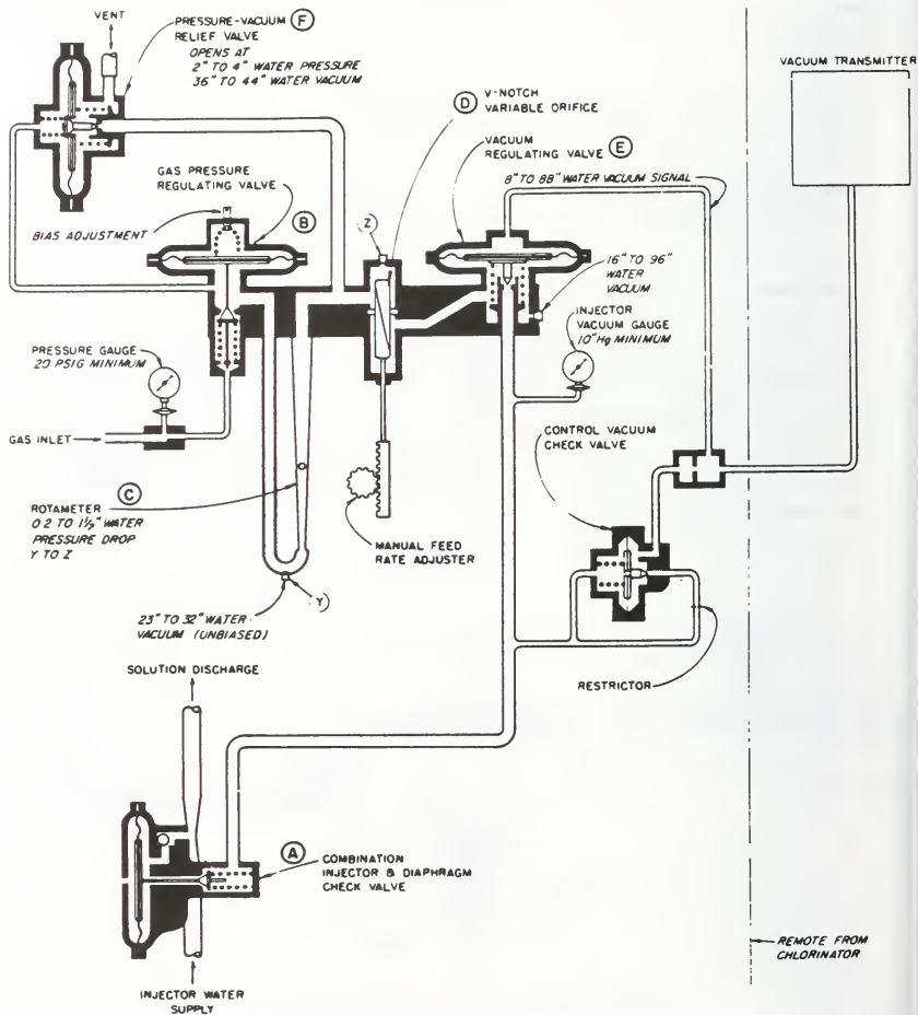
Figure 4-5 W&T V-NOTCH CHLORINATOR
