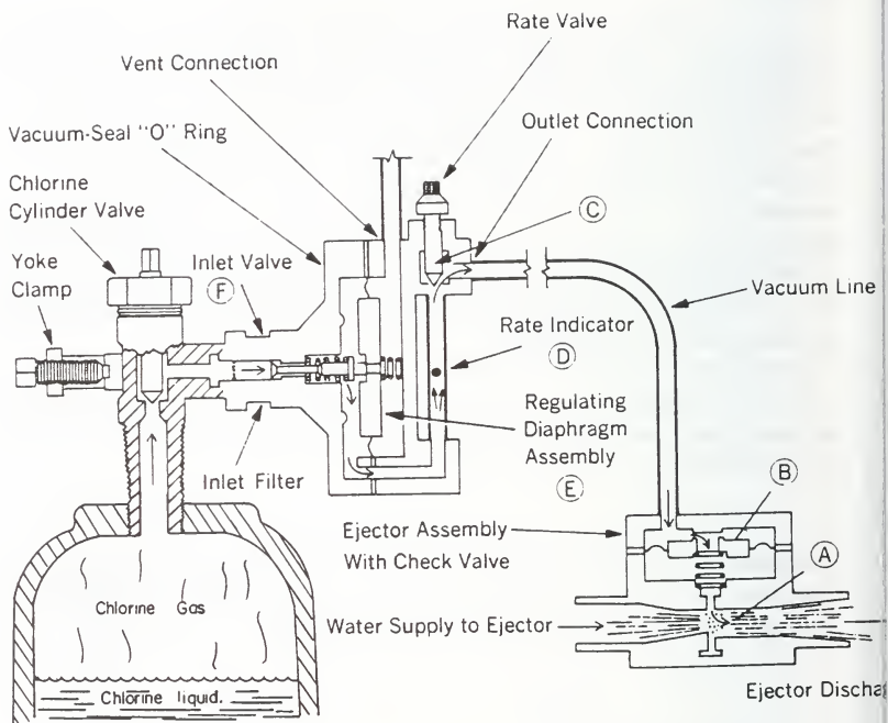
FIGURE 4-3 ADVANCE GAS CHLORINATOR
