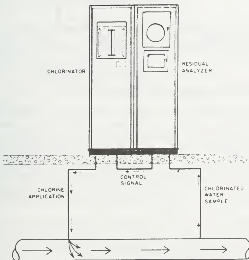
Figure 5-3 CLOSED LOOP CONTROL
