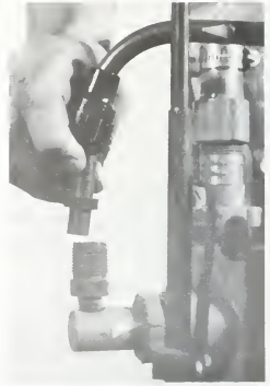
Fig. 7-2 Lift tubing from fitting.
