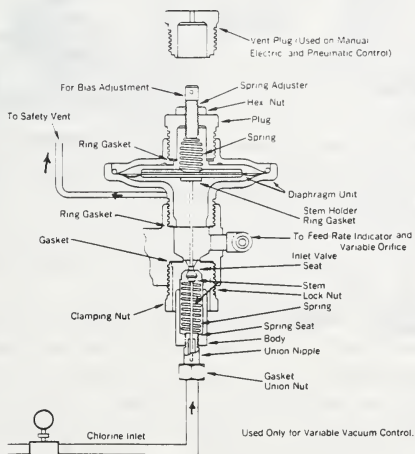
Figure 4-4 CHLORINE PRESSURE REGULATING VALVE
