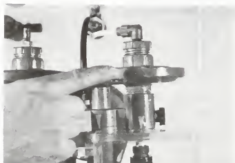
Figure 4-9 VACUUM REGULATING VALVE 180 KG CAPACITY CHLORINATOR
