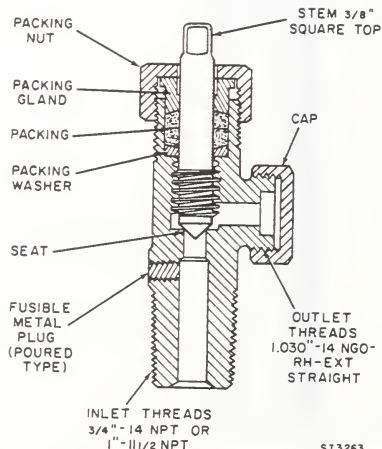
Figure 3-2 Chlorine Institute Standard Cylinder Valve 3-2
