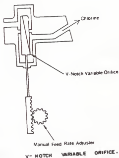
Figure 4-2 TYPES OF VARIABLE ORIFICE CONTROL
