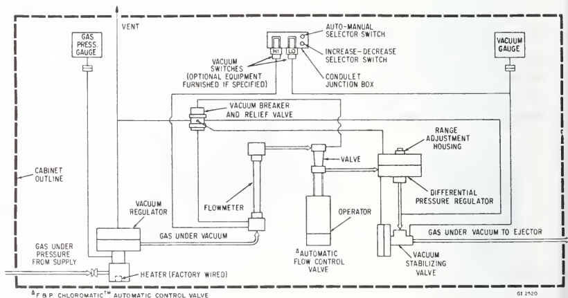
Figure 4-11 FISCHER & PORTER CHLORINATOR UPPER - SHOWING INSTALLATION LOWER - CABINET INTERIOR
