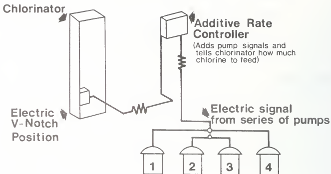
Figure 5-2 OPEN LOOP CONTROL
