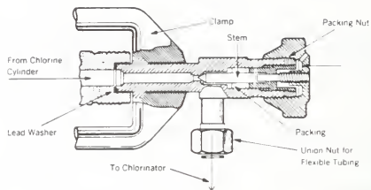
Figure 2-2 Yoke Type Auxiliary Cylinder Valve
