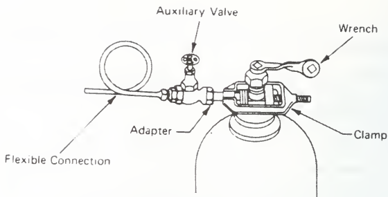
Figure 3-4 CYLINDER CONNECTION
