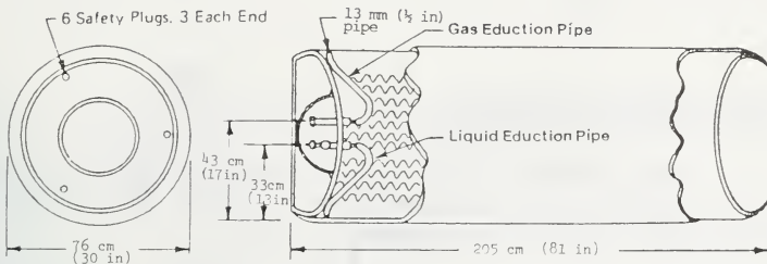
Figure 3-5 CROSS SECTION OF TON CONTAINER
