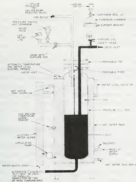
Figure 3-8 Chlorine Evaporator
