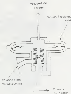
FIGURE 4-8 VACUUM REGULATING VALVE
