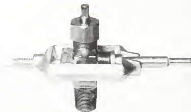
Figure 3-3 Captive yoke Auxiliary Cylinder Valve
