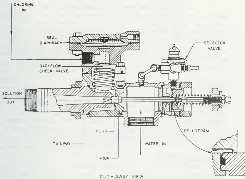
Figure 4-1 INJECTOR
