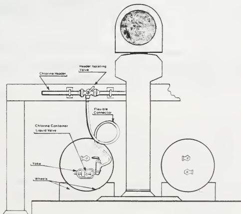
Figure 3-7 TYPICAL ONE-TON CYLINDER HOOK-UP WITH SCALES
