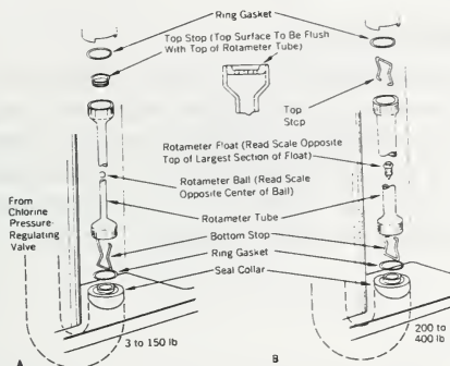
Figure 4-6 ROTAMETER
