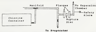
Figure 6-1 RUPTURE DISC
