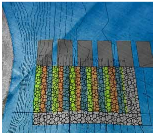
Lake Sturgeon spawning reef plan.
