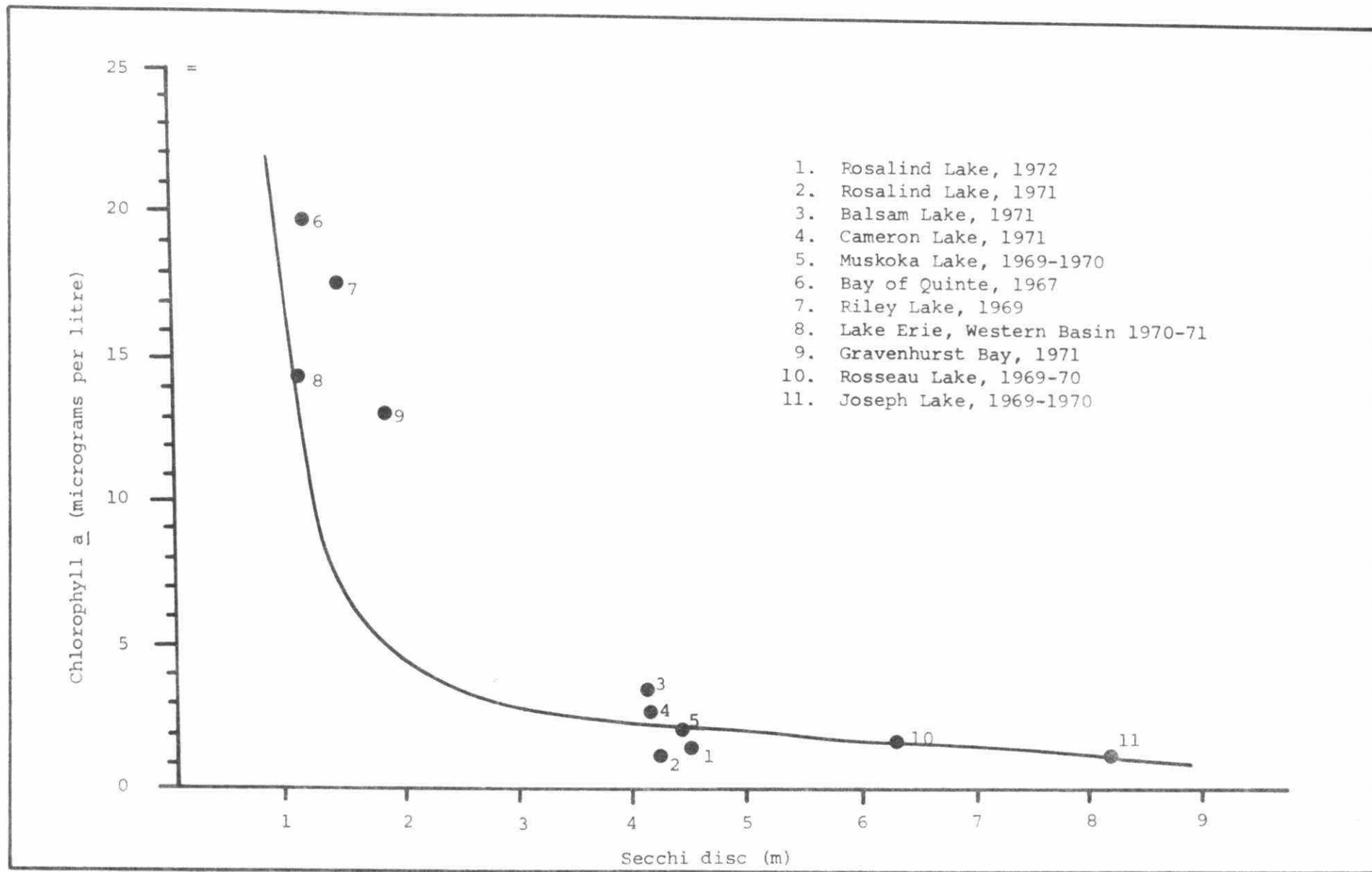
Figure 2: The relationship between chlorophyll a and Secchi disc for Rosalind Lake 1971 and 1972 and for a number of other well-known recreational lakes in the province. All data are yearly means.
