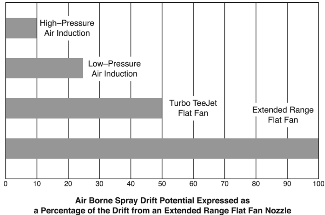
FIGURE 2–1. Conventional vs. Air Induction Nozzles.
